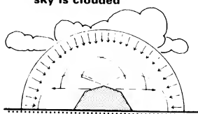
⑥ Cross-section of a house planned only for the receipt of diffuse radiation (cloudy sky)
